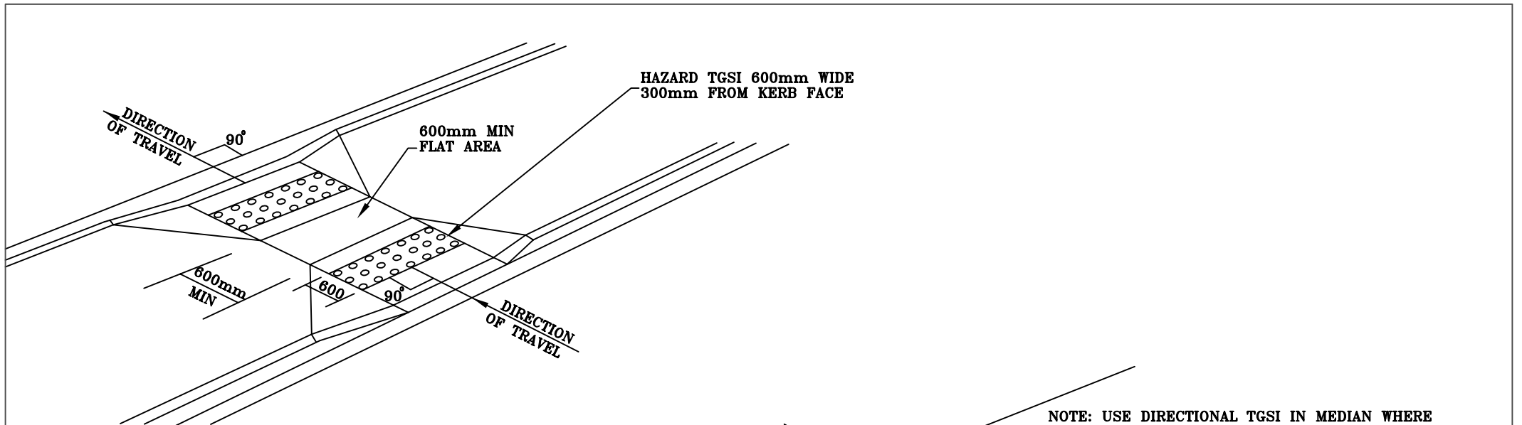
FIG 5. MEDIANS 2.4m WIDE AND GREATER REFER TO FIG. 3 FOR MEDIANS UNDER 2.4m WIDE
