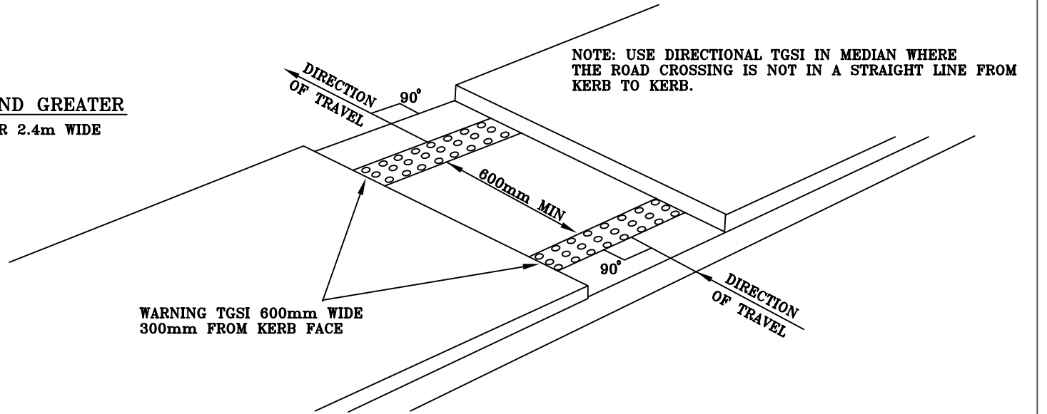
FIG 6. CUT THROUGH MEDIANS 2.4m WIDE AND GREATER REFER TO FIG. 3 FOR MEDIANS UNDER 2.4m WIDE
