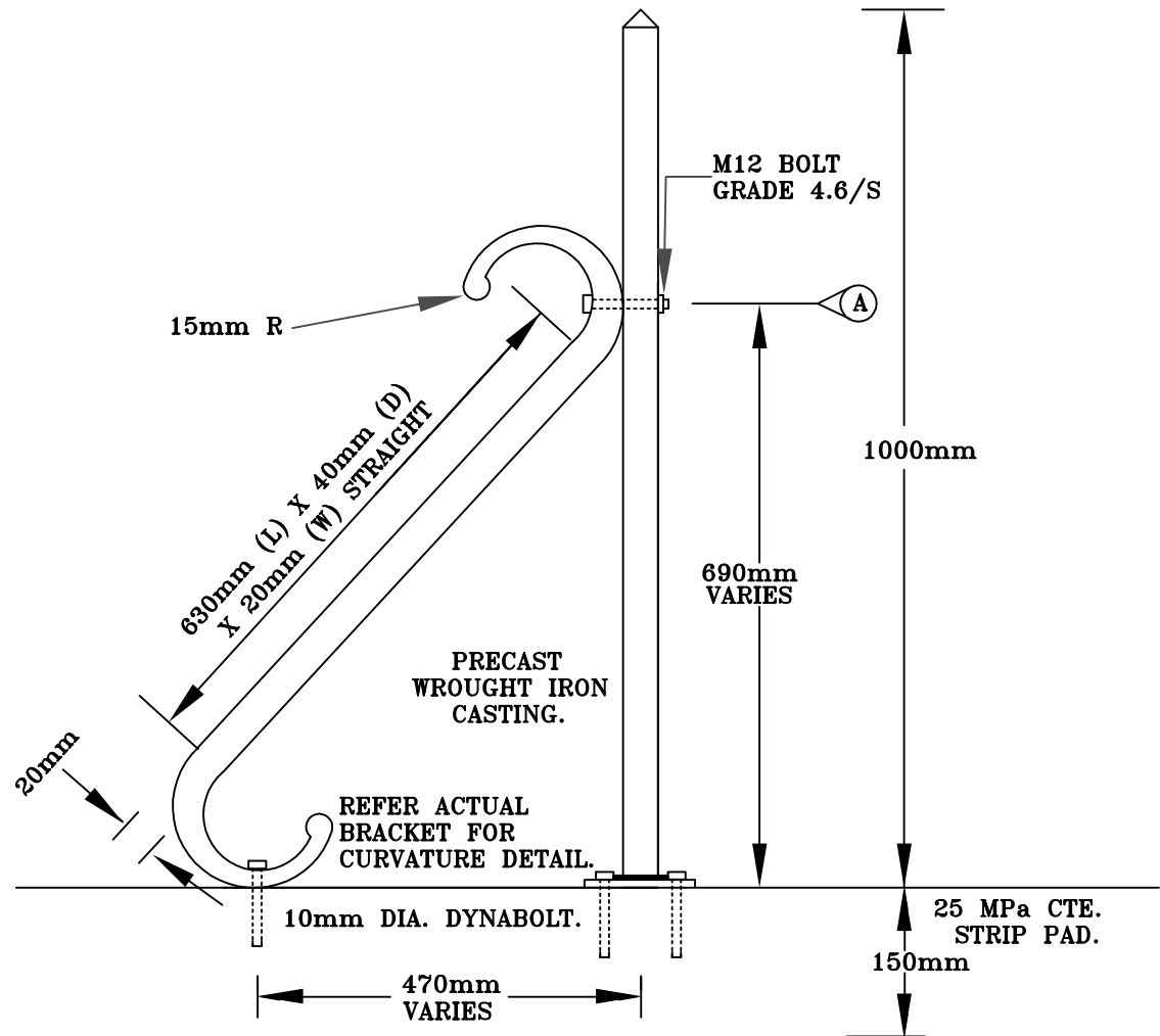
SPIRAL BRACKET DETAIL D (SOLID STEEL)
