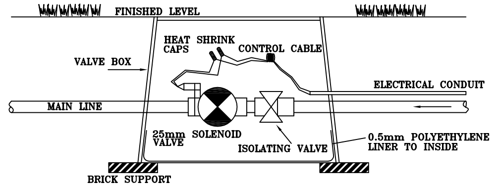
IRRIGATION SOLENOID VALVE ASSEMBLY DETAIL
