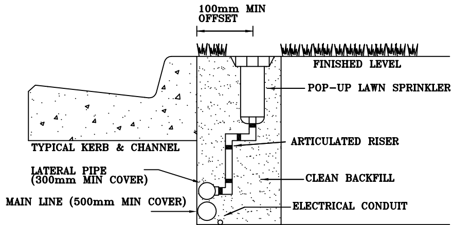
IRRIGATION POP-UP SPRAY DETAILS
