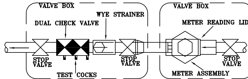
IRRIGATION METER & BACKFLOW PREVENTION DEVICE DETAIL
