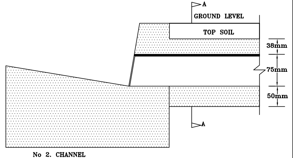
SECTION OF KERB AND CHANNEL
