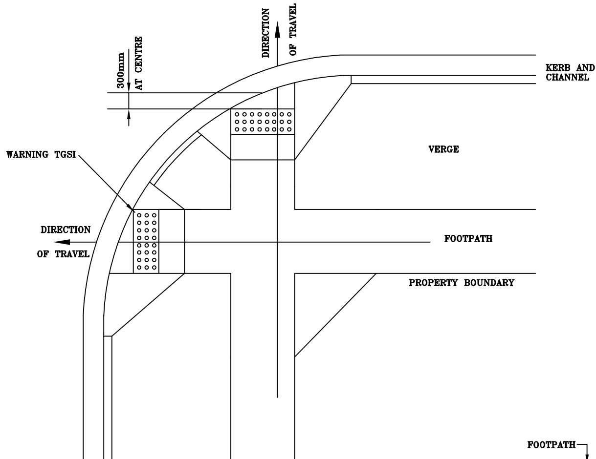
FIG 2. KERB RAMPS AT RIGHT ANGLE CORNER
