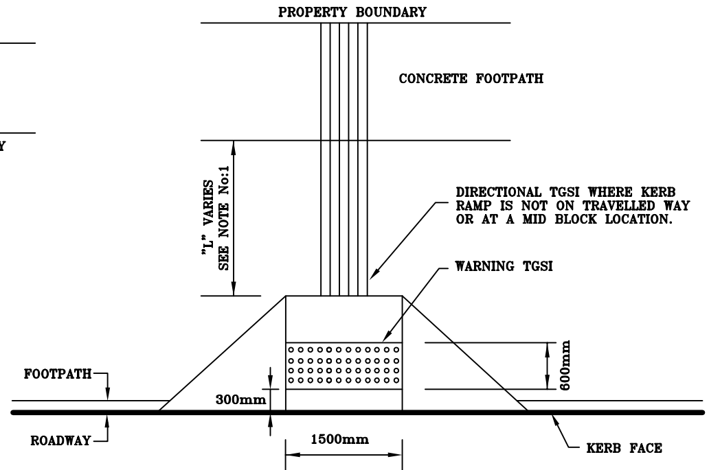
FIG 1. RIGHT ANGLE KERB RAMP
